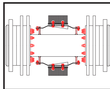
IPHS 2-4 Spring Mounted Brushes
