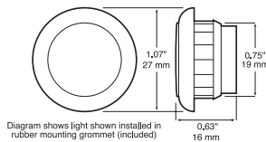
Diagram shows light shown installed in rubber mounting grommet (included)
